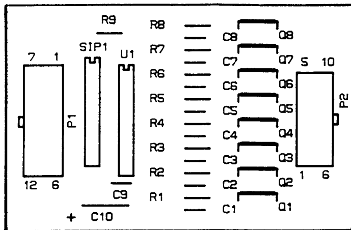
AUXILIARY DRIVER BOARD (A11) PARTS LIST
