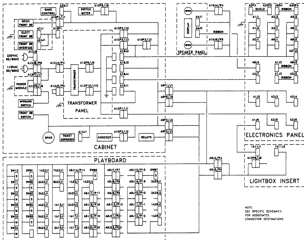
FIGURE 1. INTERCONNECTION DIAGRAM
