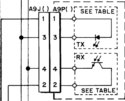
OPTO LED TRANSMITTER BOARD (TX) SCHEMATIC DIAGRAM AND OPTO PHOTOTRANSISTOR RECEIVER BOARD (RX) SCHEMATIC DIAGRAM
