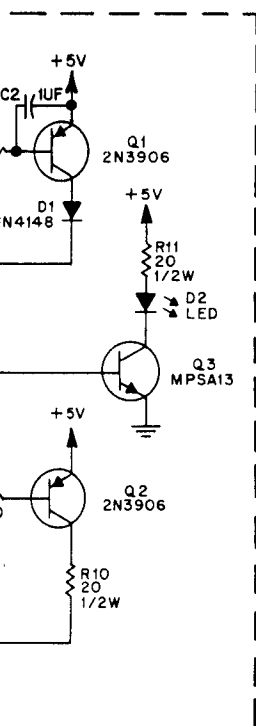
SCHEMATIC DIAGRAM AUXILIARY DRIVER BOARD (A11) COMPONENT LOCATION
